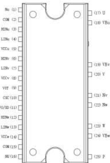
Fig 1: Internal circuit
